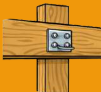
HEAVY BEAMS
